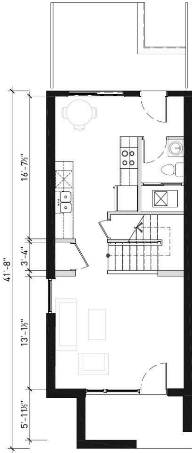
1 UNIT A - FIRST LEVEL SCALE: 1/8"=1'-0"
