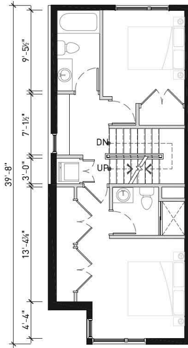
2 UNIT A - SECOND LEVEL SCALE: 1/8"=1'-0"
