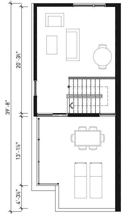
3 UNIT A - THIRD LEVEL SCALE: 1/8"=1'-0"
