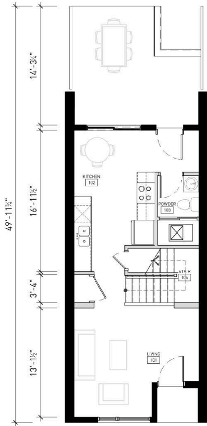
1 UNIT B - FIRST LEVEL SCALE: 1/8"=1'-0"
