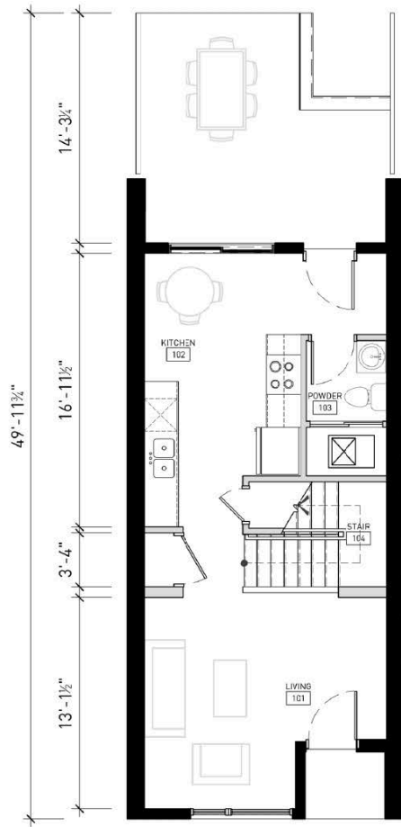
1 UNIT B - FIRST LEVEL SCALE: 1/8"=1'-0"
