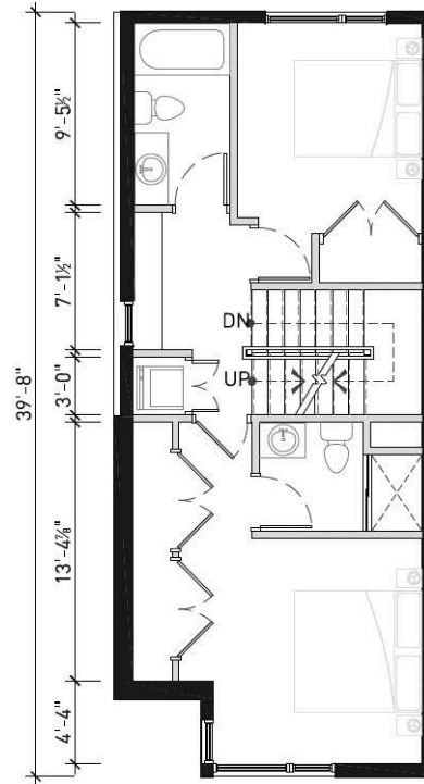
2 UNIT A - SECOND LEVEL SCALE: 1/8"=1'-0"
