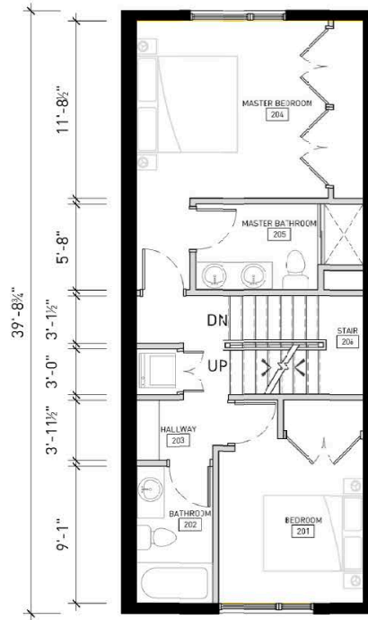
2 UNIT B - SECOND LEVEL SCALE: 1/8"=1'-0"
