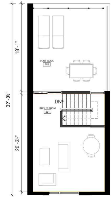
3 UNIT B - THIRD LEVEL SCALE: 1/8"=1'-0"
